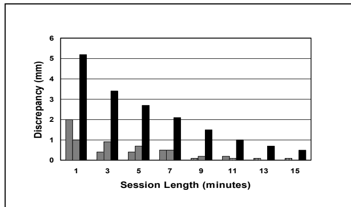
Figure 8-5. Convergence of coordinate component discrepancies to the true position with a simulated displacement of 2.5 mm. For each session, the components are plotted north, east, and height respectively.
